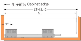
外置抽屉 Standard drawer
